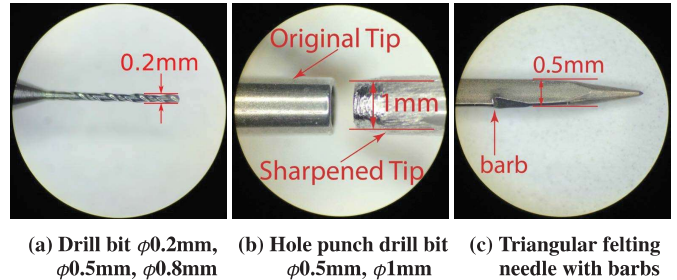
Figure 3. Hole opener
