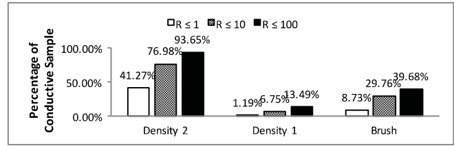
Figure 7. Percentage of conductive samples
