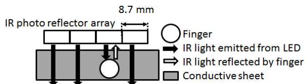
Figure 7. Principle of an IR photo reflector array to detect one-dimensional finger position.
