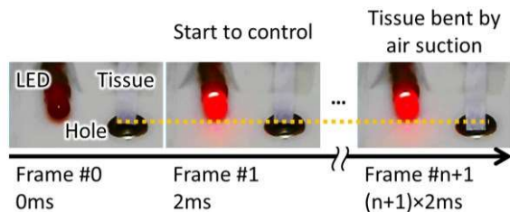
Figure 3. The setup to investigate the latency between the microcontroller's order and the generation of the suction force. Typical duration is 10ms ( \#n=5 with a 500 fps).
