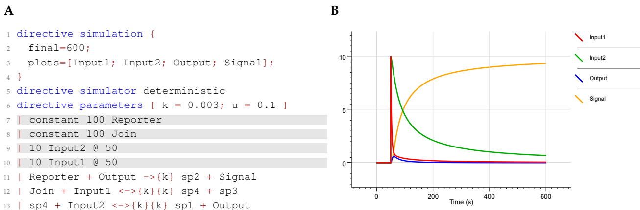
Figure 10: Example initial conditions. A CRN program from Figure 9, updated with constant and delayed initial conditions. The Reporter and Join species are assumed to be in excess, however they will be consumed over time if they are not fixed as constant, slowing down the release of the Signal strand. Fixing these species as constant is a convenient way to study the effect of species loss over time on system kinetics. In addition, in a laboratory experiment the Reporter and Join species will typically be mixed in solution beforehand, prior to adding the Input1 and Input2 species a short time later. This can be modelled by delaying the addition of the two input species. In this example both species are added after 50 time units. B Simulation results for the CRN program in (A). We observe a discrete spike in the concentrations of both inputs after 50 time units. The Reporter and Join species remain constant at 100 throughout the duration of the simulation (not shown), however this does not seem to significantly alter the system dynamics, suggesting that species loss does not play a key role in this particular simulation.
