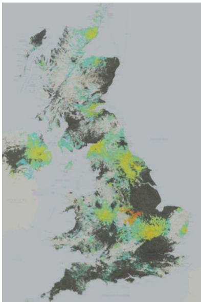
Figure 01: Use of Channel 22 – showing protected areas in black and permissible WSD power levels in varying shades
