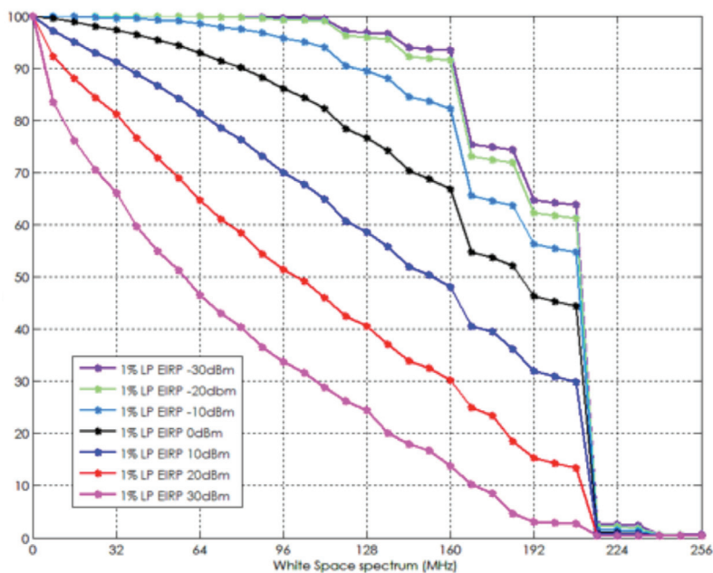
Figure 08: UK White space availability per household as a function of WSD EIRP
