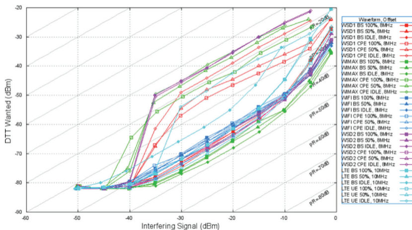
Figure 23: C/I for a poorly performing receiver 8 MHz offset
