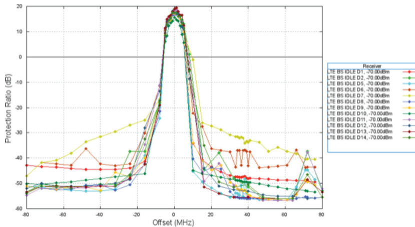
Figure 22: Protection Ratio for all Receivers LTE Idle. Wanted signal -70 dBm.
