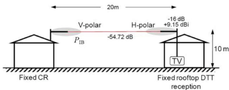
Figure 20: Reference geometry 2 for a fixed 10m WSD device to a 10 m DTT antenna
