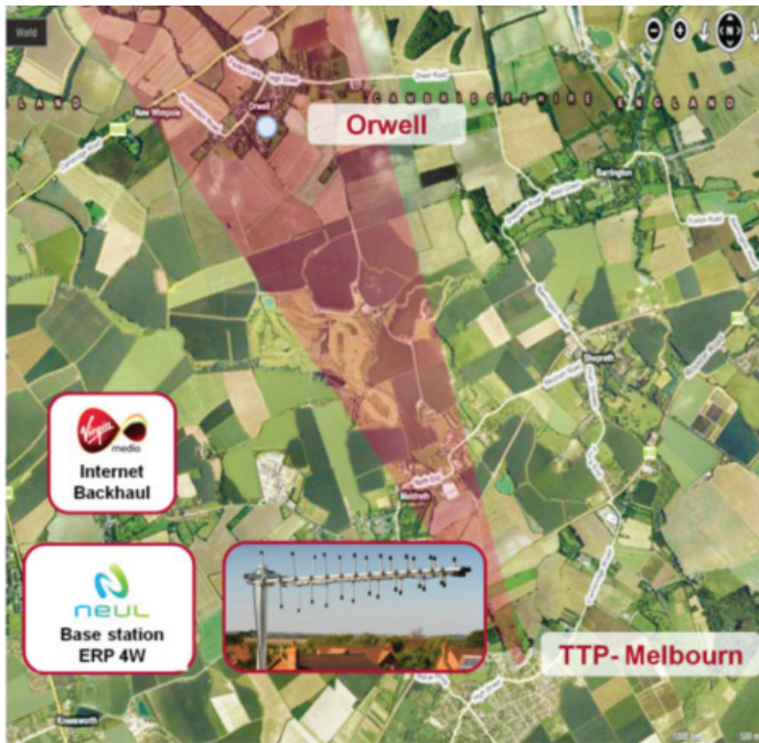
Figure 16: The TTP Base station providing broadband service to Orwell
