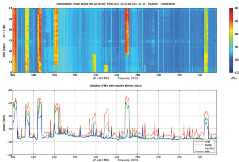
Figure 06: Long term plots compiled from the monitoring data
