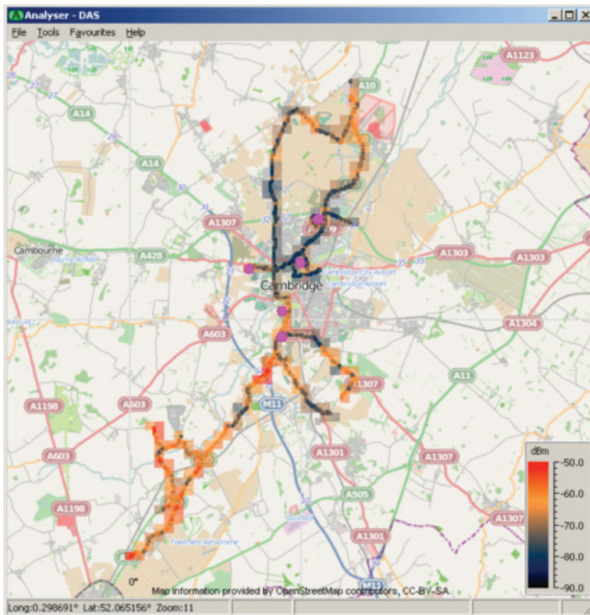
Figure 05: Locations of CRFS fixed monitoring nodes (pink markers), and combined route of mobile surveys (coloured tracks, showing peak power in 470 – 862 MHz band).
