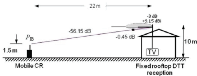
Figure 19: Reference geometry 1 for a 1.5m WSD device to a 10 m DTT antenna
