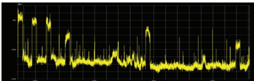
Figure 07: An example spectrum scan taken using a mobile monitoring node
