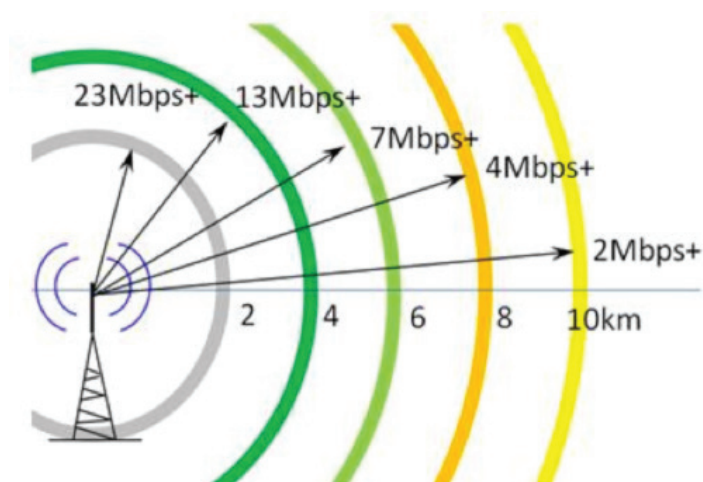
Figure 18: Analysis based on Shannon +3 dB margin and 65 % PHY>MAC> Network packet efficiency with 60/40 downlink vs uplink timings
