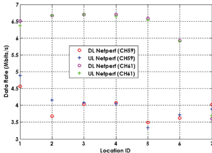
Figure 15: Throughput comparison between Channel 59 and Channel 61
