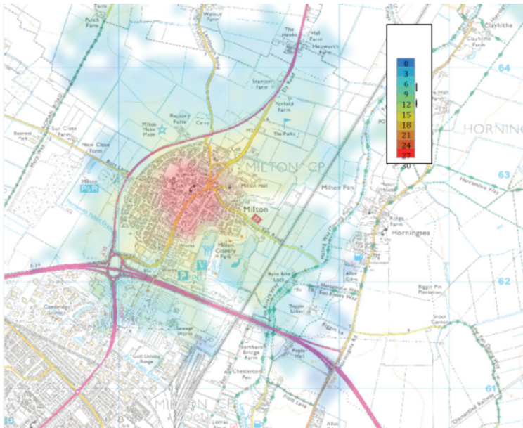
Figure 13: UKPM Coverage Prediction for CH 59 BS Coverage
