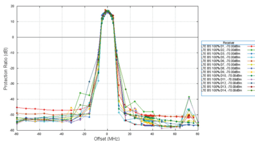
Figure 21: Protection Ratio for all Receivers LTE 100 % BS. Wanted signal -70 dBm
