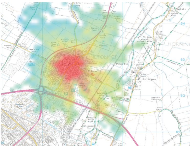
Figure 14: UKPM Coverage Prediction for CH 61 BS Coverage
