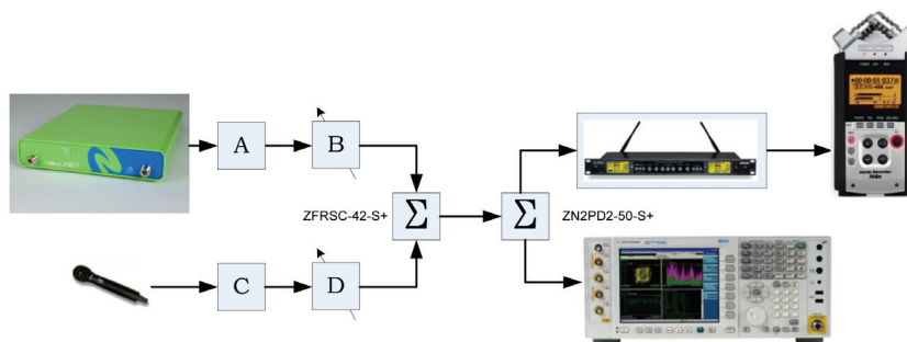
Figure 24: Radio Microphone Bench Test Configuration
