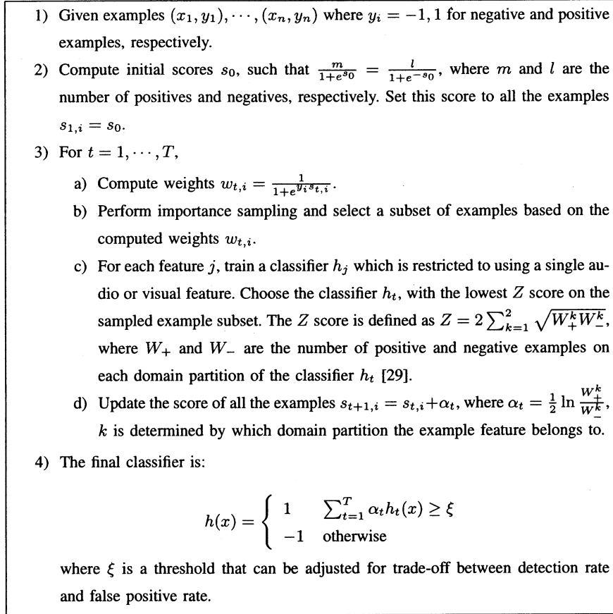
Fig. 6. Flow of the Boosting training algorithm.
