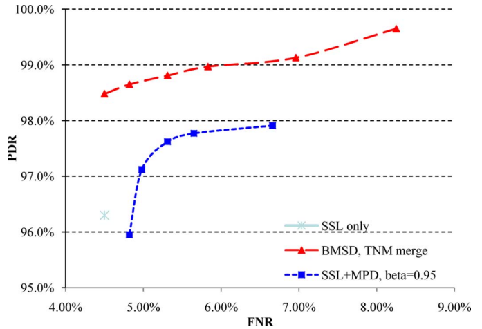
Fig. 12. Person detection performance of various algorithms on the test data set.
