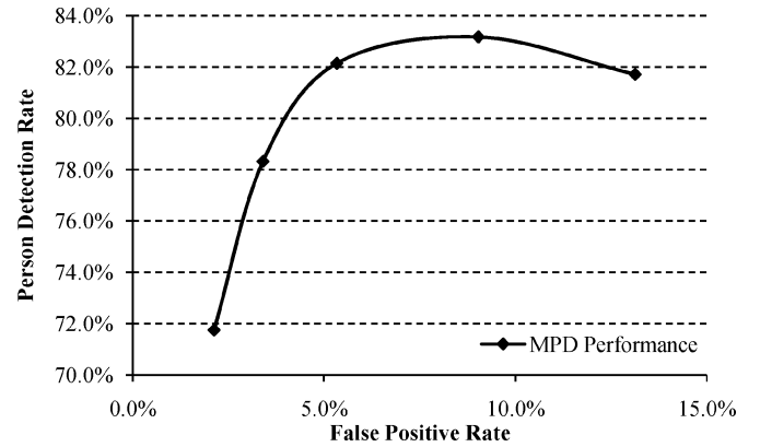
Fig. 9. Performance of the MPD detector on the test data set.
