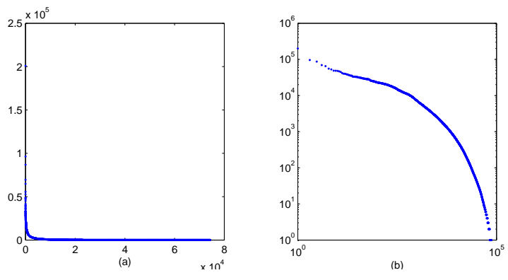
Figure 2: Distribution of the number of authors in (a) linear (b) log-log scale
