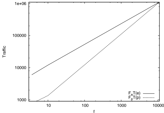
(b) Maximum forwarding load.
