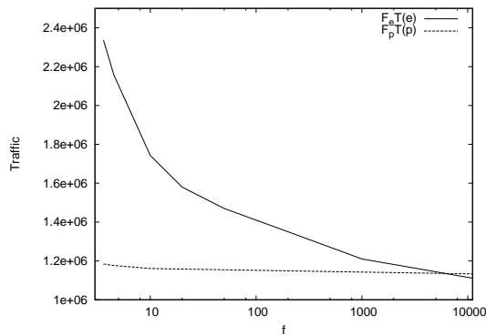
(a) Message overhead.
