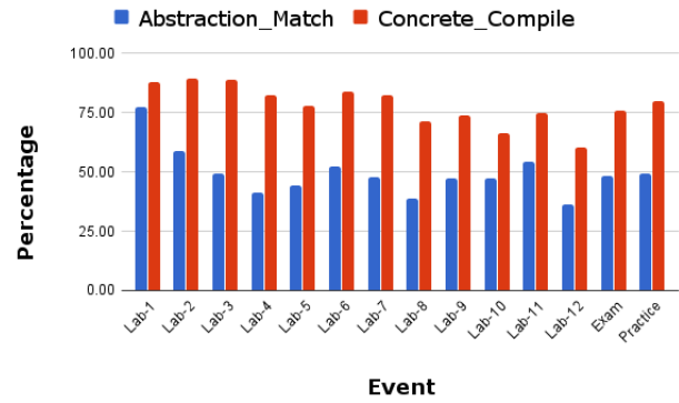
Figure 5: Overall accuracy of TRACER, shown per lab. TRACER is robust to handle compiler errors occurring across all labs. Even on erroneous programs dealing with advanced concepts such as pointers and recursion, TRACER is able to consistently achieve high repair rate.
