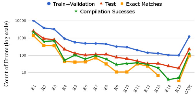
(b) Compiler Errors Plot
