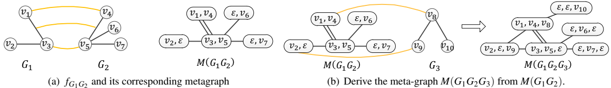
Figure 6. An example of meta-graph and its iterative matching operation. \epsilon represents a null node.
