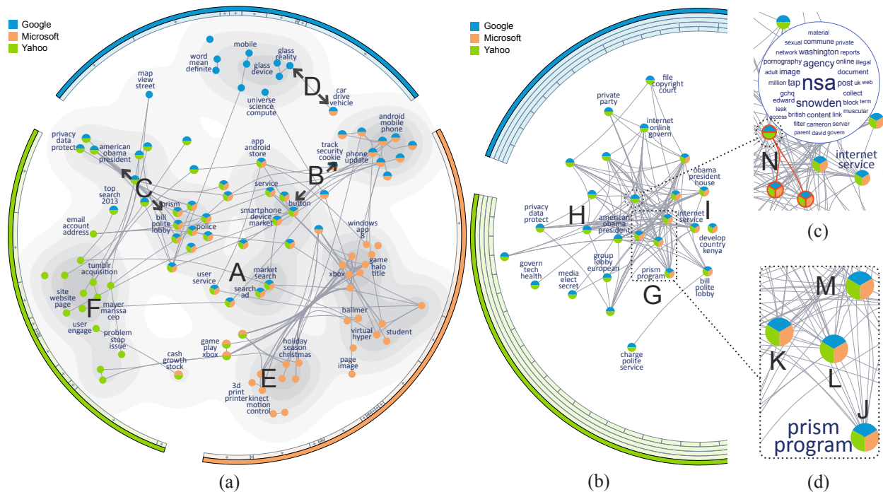
Figure 1. TopicPanorama visualization: (a) a full picture of topics related to Google, Microsoft, and Yahoo; (b) government related topics; (c) NSA Prism spying scandal shared by Google and Yahoo; (d) NSA Prism spying scandal shared by the three companies. Notations A-I represent different groups of topics and J-N represent different topics.
