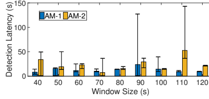
Fig. 32: Detection delay v.s. window size.
