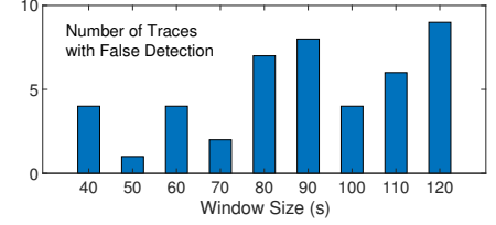
Fig. 33: False detection v.s. window size.
