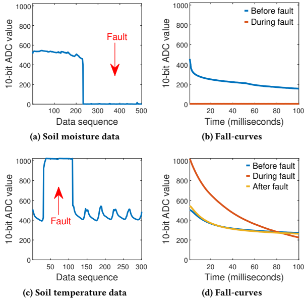
Figure 15: Stuck-at fault and its corresponding Fall-curves.
