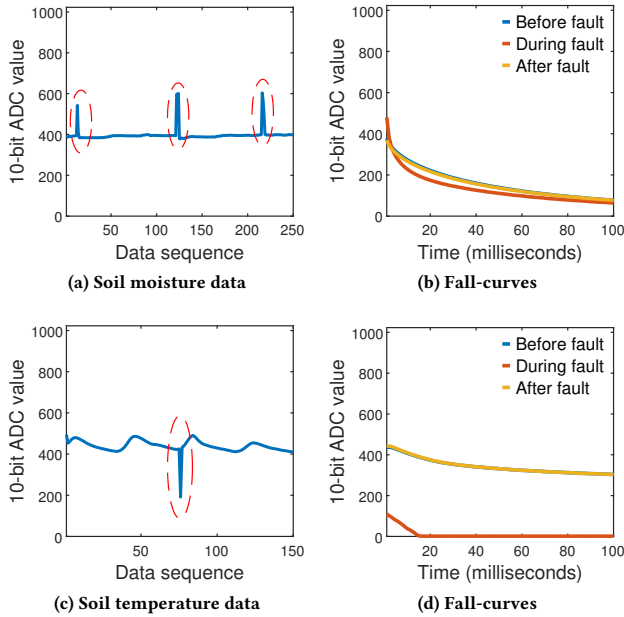
Figure 13: Short fault and its corresponding Fall-curves.
