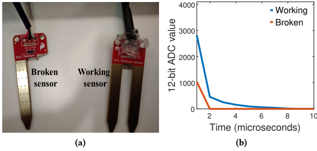
Figure 6: Manually injected faults: Soil moisture.
