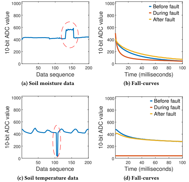
Figure 14: Spike fault and its corresponding Fall-curves.
