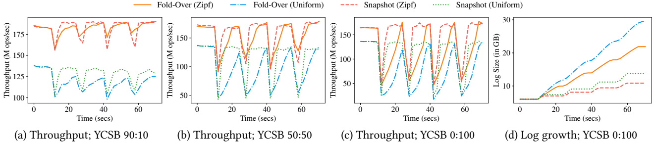
Figure 18: FASTER Throughput and Log Growth vs. Time; Log-only Fold-over and Snapshot Commits
