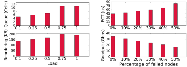
Figure 16: Max queue size and max cell reordering vs. traffic load.
