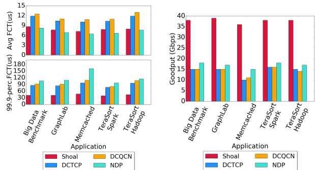
(a) Flow completion time. (b) Average flow goodput.
