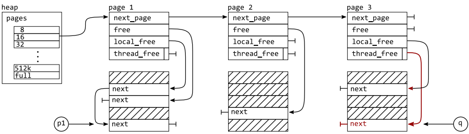
Fig. 8. Freeing objects
