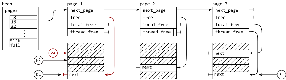
Fig. 9. Allocating objects
