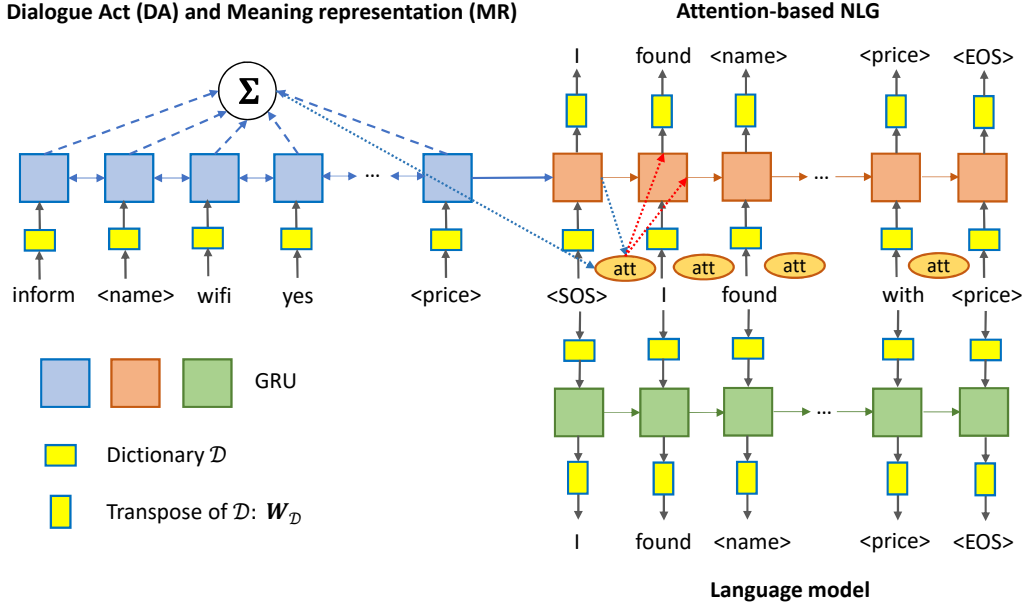
Figure 1: NLG-LM model structure. The encoder takes dialogue act (DA) and meaning representations (MR) as input. The decoder for NLG applies attention on encoder outputs, and the decoder for language modeling shares dictionary with NLG but uses a separate GRU unit.
