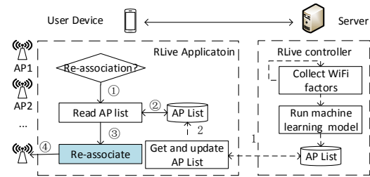
Fig. 11. Working process of RLive.
