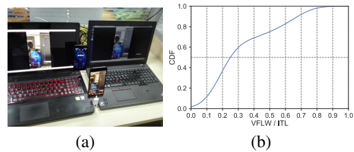
Fig. 3. (a) A pilot testbed to measure interactive latency ( i.e. , ITL ) and video frame latency over WiFi ( i.e. , VFLW ). (b) The distribution of \frac{VFLW}{ITL} , which indicates that VFLW can be the major contributor of ITL .
