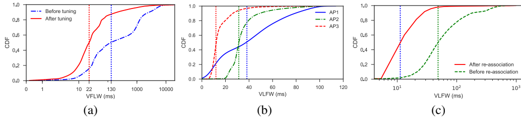
Fig. 10. (a) VFLW 's distribution before and after optimization; (b) VFLW 's distribution of three APs; (c) VFLW 's distribution before and after re-association.
