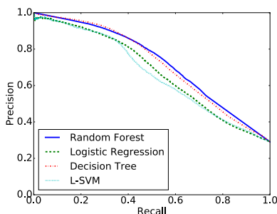
Fig. 9. Performance comparisons of different machine learning algorithms.
