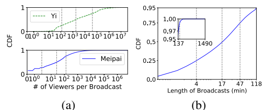
Fig. 1. Application characteristics. (a) Amount of viewers per broadcast, (b) Length of broadcasts for Meipai.
