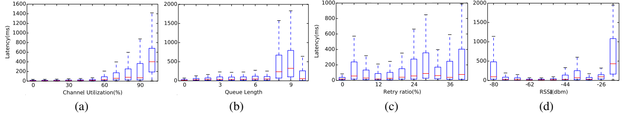
Fig. 7. Relationship between WiFi factors (x-axis) and PL's VFLW (y-axis).
