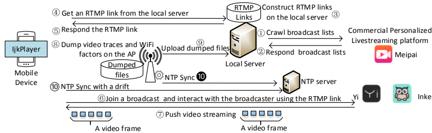
Fig. 5. LTR's detailed process for measuring PL's frame latency over WiFi (i.e., VFLW ).
