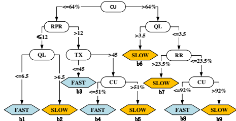
Fig. 8. Pruned Decision Tree for classifying VFLW into FAST and SLOW .
