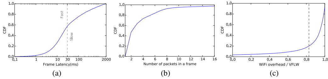
Fig. 6. (a) Distribution of the video frame latency over the WiFi hop; (b) Distribution of packet count per frame; (c) Distribution of WiFi overhead in VFLW .
