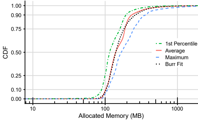
Figure 8: Distribution of allocated memory per application.
