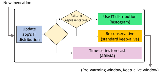
Figure 10: Overview of the hybrid histogram policy.
