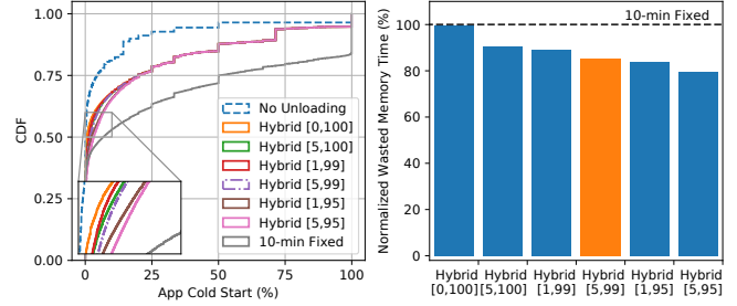
Figure 16: Wasted memory time can be significantly reduced by excluding outliers from the IT distribution.
