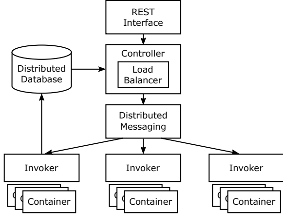
Figure 13: OpenWhisk architecture.
