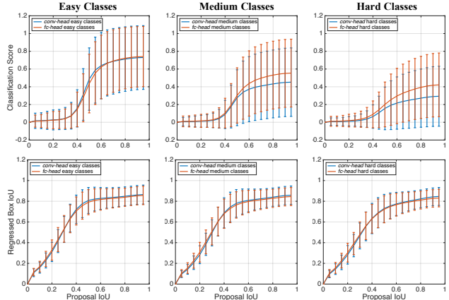
Figure A.1. Comparison between fc-head and conv-head on easy, medium and hard classes. Top row: mean and standard deviation of classification scores. Bottom row: mean and standard deviation of IoUs between regressed boxes and their corresponding ground truth.
