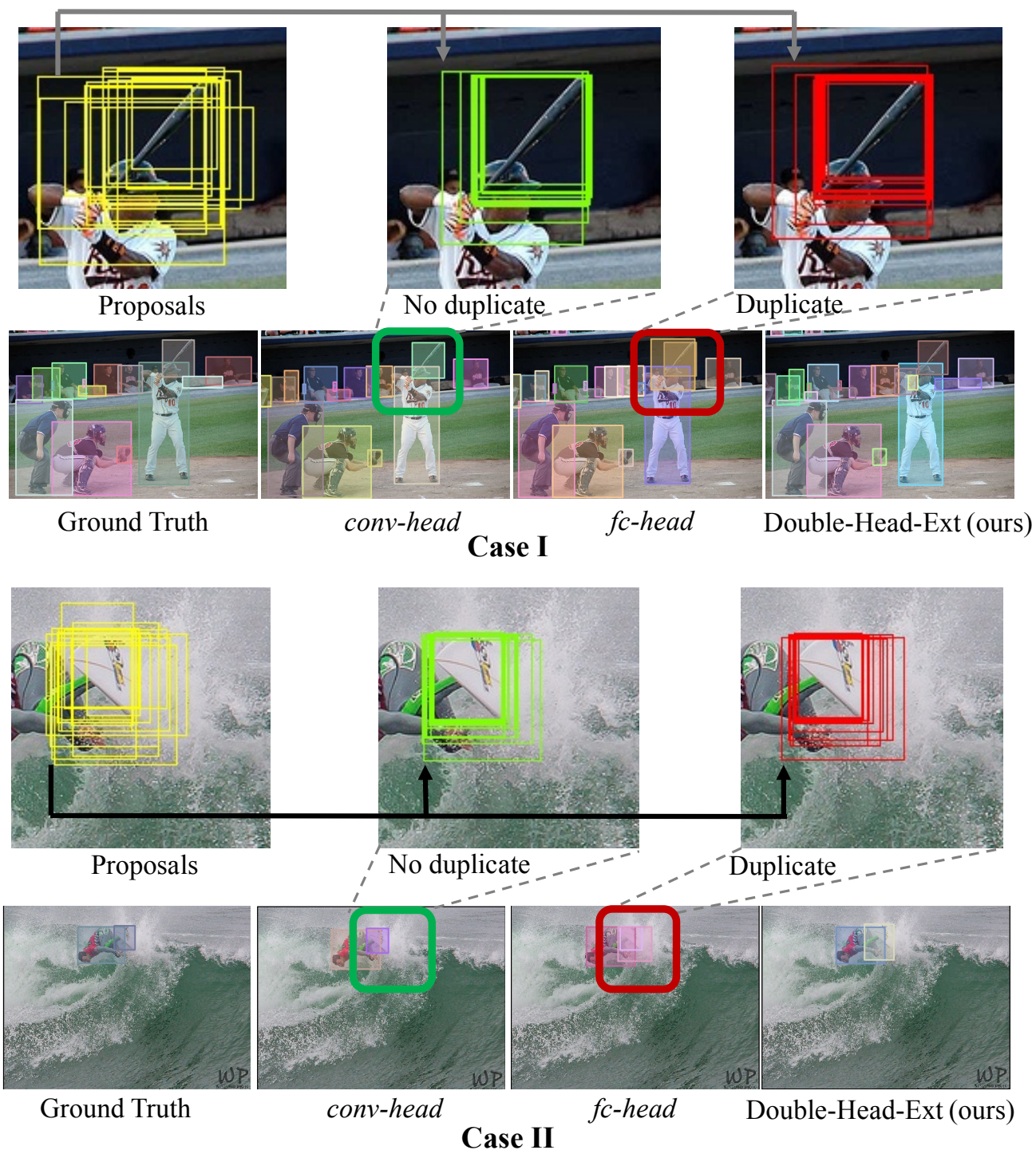
Figure A.5. conv-head is more suitable for localization than fc-head . This figure includes two cases. Each case has two rows. The bottom row shows ground truth, detection results using conv-head alone, fc-head alone, and our Double-Head-Ext (from left to right). fc-head has a duplicate detection for the baseball bat in case I and for the surfing board in case II (in the red box). The duplicate detection is generated from an inaccurate proposal (shown in the top row), but is not removed by NMS due to its low IoU with other detection boxes. In contrast, conv-head has more accurate box regression for the same proposal, with higher IoU with other detection boxes. Thus it is removed by NMS, resulting no duplication.
