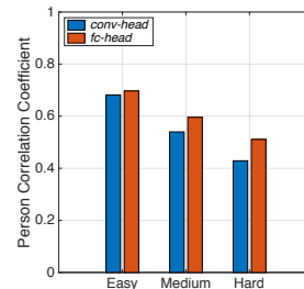
Figure A.2. Pearson correlation coefficient (PCC) between classification scores and IoUs of predefined proposals for easy, medium and hard classes.
