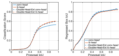
Figure A.3. Comparison of classification and bounding box regression. Left: mean of classification scores between single heads and Double-Head-Ext. Right: mean of regressed box IoUs between single heads and Double-Head-Ext.
