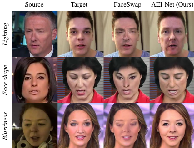
Figure 2: Failure cases of a previous method on FaceForensics++ [35] dataset. From left to right we show the input source images, the input target images, the results of FaceSwap [2], and the results of our method. FaceSwap follows the strategy that, first synthesizes the inner face region, then blends it into the target face. Such strategy causes artifacts, such as the defective lighting effect on the nose (row 1), failing to preserve the face shape of the source identity (row 2) and the mismatched image resolutions (row 3). While our method addresses all these issues.
