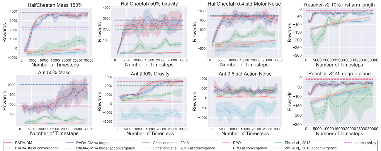
Figure 2. We plot the learning curves across 5 random seeds on a number of tasks. The title of each plot corresponds to the perturbation in the target domain, e.g., HalfCheetah Mass 150% means in mass of the agent in the target domain is 150% of that in the source domain.
