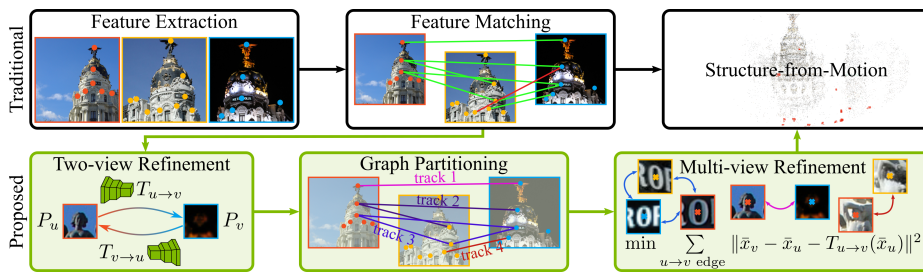
Fig. 2. Overview of the proposed method. Our method operates on the tentative matches graph (with patches as nodes P_u, P_v and matches as edges) without knowledge of scene and camera geometry. A neural network is used to annotate the edges of this graph with local geometric transformations ( T_{u \rightarrow v}, T_{v \rightarrow u} ). Next, the graph is partitioned into tracks, each track containing at most one patch from each image. Finally, the keypoint locations x_u, x_v are refined using a global optimization over all edges.
