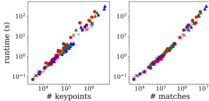
Fig. 11. Graph optimization runtime. The runtime is plotted as a function of the number of keypoints and matches. We respect the color coding from the main paper: SIFT [24], SURF [7], D2-Net [12], R2D2 [31], SuperPoint [10], and Key.Net [6].
