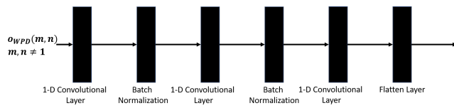
Figure 10: CNN stack
