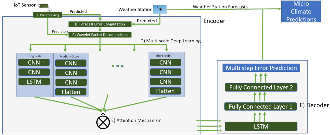
Figure 1: DeepMC architecture for the multi scale encode-decoder deep learning system. The architecture consists of 6 distinct parts- A) The preprocessor, B) Forecast error computation, C) Wavelet packet decomposition, D) Multi-scale deep learning, E) Attention Mechanism, F) Decoder. The attention mechanism is depicted in Figure 3.
