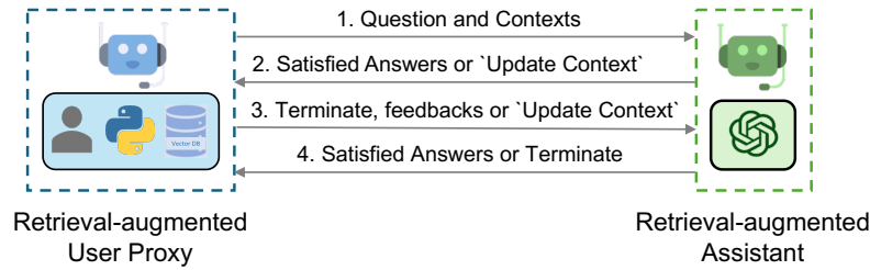
Figure 7: Overview of RAG Chat which involves two agents, including a RAG User Proxy and a Retrieval-augmented Assistant. Given a set of documents, the Retrieval-augmented User Proxy first automatically processes documents—splits, chunks, and stores them in a vector database. Then for a given user input, it retrieves relevant chunks as context and sends it to the Retrieval-augmented Assistant, which uses LLM to generate code or text to answer questions. Agents converse until they find a satisfactory answer.
