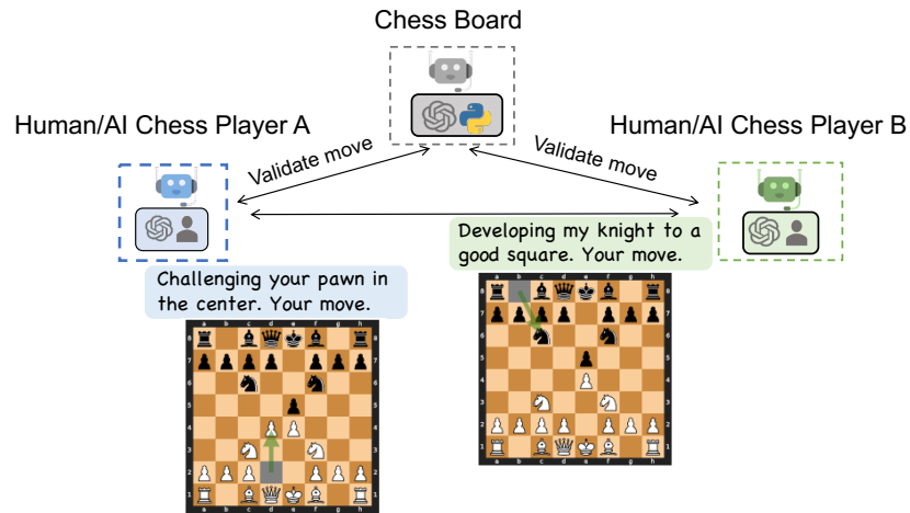
Figure 14: Illustration of our conversational chess application. The application can support various scenarios, as each player can be an LLM-empowered AI, a human, or a hybrid of the two. Here, the board agent maintains the rules of the game and supports the players with information about the board. Players and the board agent all use natural language for communication.
