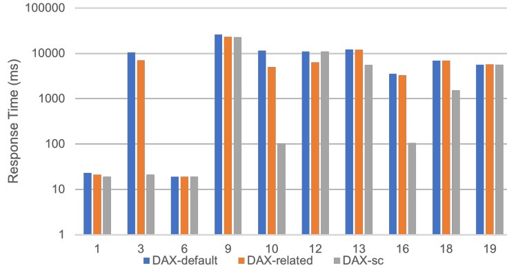
Figure 6: Impact of Rewrite Rules (TPC-H benchmark)
