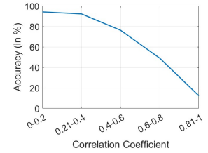
(b) Collision resolution accuracy by the correlation coefficient of Doppler signatures
