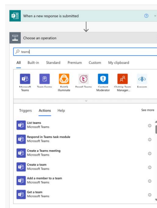
Fig. 1: Action selection interface in the Microsoft Power Automate platform. For each action in a workflow, the user must manually navigate to the desired action.
