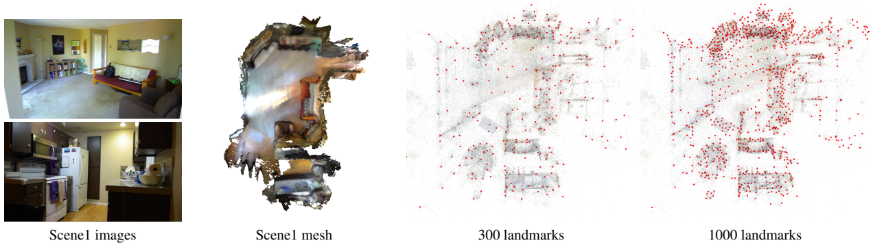
Figure 4. The top view of the mesh and 3D SfM point cloud from scene1, shown with the overlaid scene landmarks (red points). The sets of 300 and 1000 landmarks respectively are both computed by the existing selection method [11]. The image on the right shows that a higher number of landmarks provides denser scene coverage. We show later that it leads to an improvement in camera pose accuracy.
