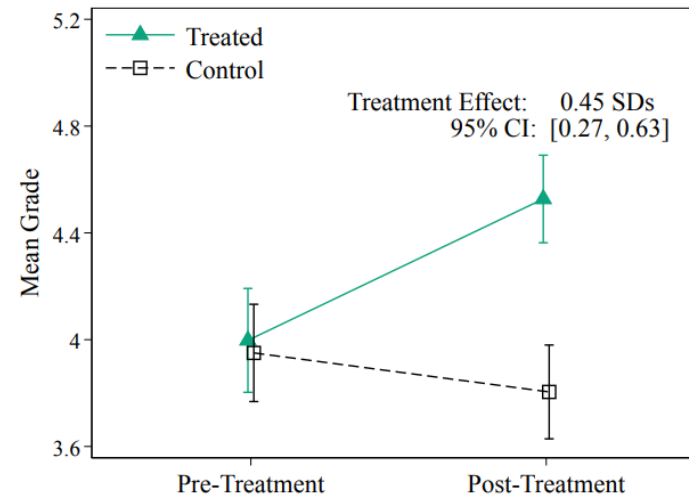
Quality of output (Treated = using ChatGPT) (Noy & Zhang 2023)
