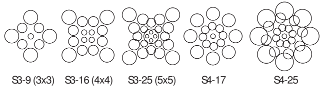
Figure 12. Examples of learned configurations of summation regions for the S3 and S4 blocks. These diagrams are to scale and circles represent the size of the Gaussian weighting function at each sample. The lattice positions and Gaussian sizes were initialized to be uniform. From left to right, the number of free parameters was 5, 7, 12, 6, and 9.
