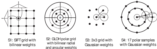
Figure 3. Examples of the different spatial summation blocks. For S3 and S4, the positions of the samples and the sizes of the Gaussian summation zones were appropriately parameterized.
