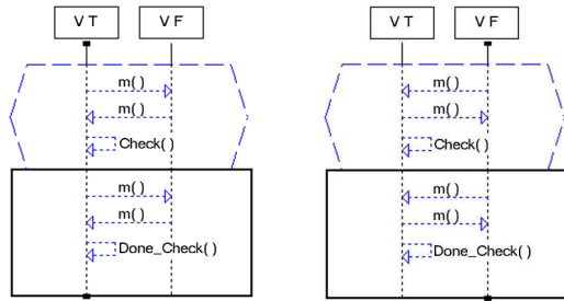
(a) Type 2A charts: for “resending” the last value, if true, of each variable v after a Check v_t \xrightarrow{\text{Check}} v_t message.
