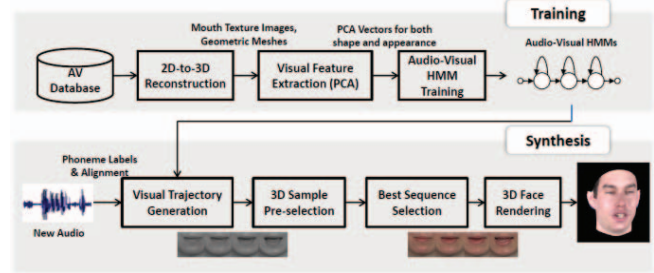
Fig. 1. Training and synthesis for 3D photo-realistic lip-sync animation.
