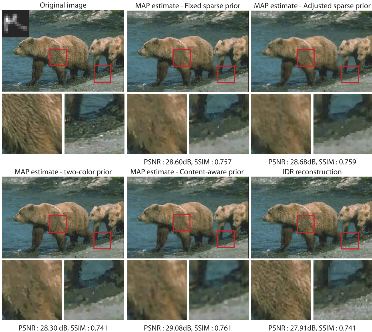
Fig. 8. We compare the performance of IDR against four other competing methods. 1) A MAP estimator with a sparse gradient prior [21]. 2) A MAP estimator with a sparse prior adapted to each segment. 3) A MAP estimator with a two-color prior [16]. 4) A MAP estimator with a content-aware image prior. The red boxes indicate the cropped regions. Although the PSNR and the SSIM of our results are often lower than those using MAP estimators, IDR restores more visually pleasing textures (see bear furs).
