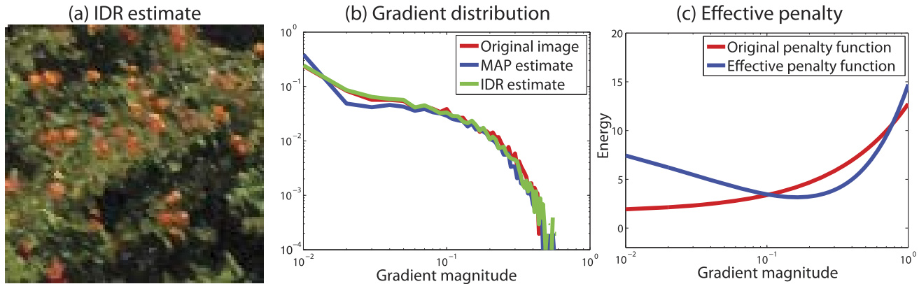
Fig. 4. The IDR deconvolution result. (a) shows the deconvolved image using IDR and (b) compares the gradient distribution of images reconstructed using the MAP estimator and IDR. (c) The effective penalty after convergence (i.e., w_1 \lambda_D |\nabla I|^{\gamma_D} + w_2 \sum_{i=1}^{10} \frac{1}{N} \ln(\frac{q_E(\nabla I)}{q_D(\nabla I)}) ) penalizes gradients with small and large magnitude more than gradients with moderate magnitude. q_D is set to the ground truth distribution.
