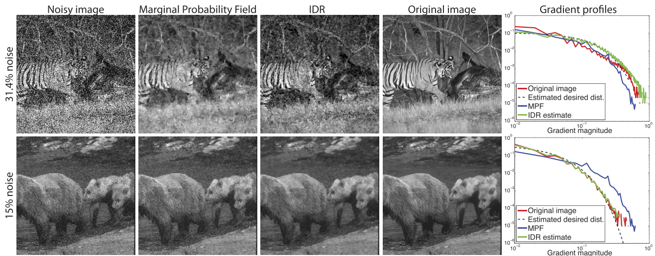
Fig. 10. Comparing the denoising performance of IDR to the marginal probability field [39]. IDR generates a better rendition of the spatially variant texture.
