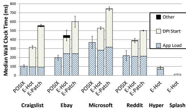
Figure 6: App Startup Latency. Four web apps, a native game (Hyperoid), and a splash screen. For the web apps “App Load” is the time to fetch and render the HTML content. Error bars show standard deviations of total time over 5 runs.
