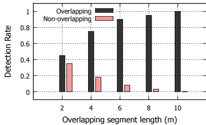
Figure 21: Overlapping segment detection results.
