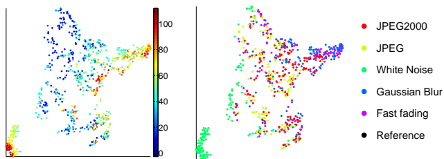
Figure 6. The t-SNE embedding of the concatenated feature space. In both images, each point corresponds to an image. In left image, color encodes subjective quality score; in right image, color encodes distortion type. This embedding verifies that our designed feature set naturally clusters images degraded in a similar way and by a similar extent.
