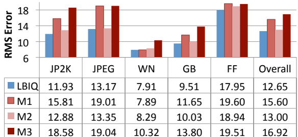
Figure 7. Median root mean square error between prediction and subjective score (lower means better). Much of the strength of our LBIQ measure comes from the second kernel machine which trains on cross-scale histogram and statistics of wavelet coefficients. However, the combination of all three machines decreases the Median RMSE up to 1.
