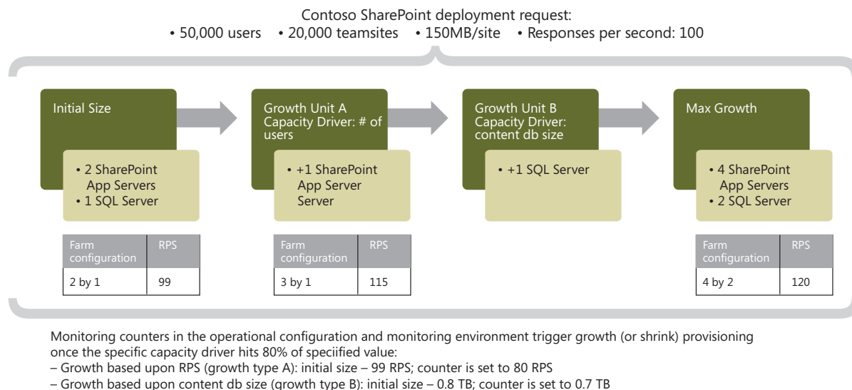
Figure 6: Scale-Units Grow
