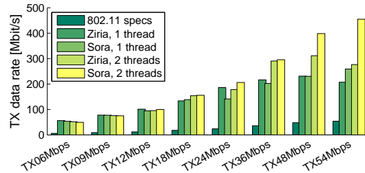
Figure 6: WiFi throughput
