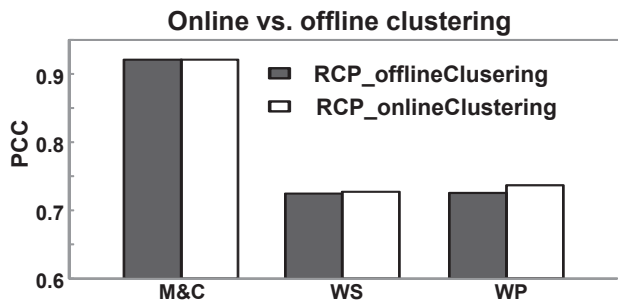
Figure 5: Performance of RCP with online/offline clustering
