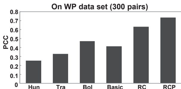
Figure 6: Performance comparison on WP
