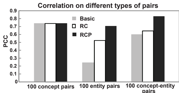
Figure 7: Performance comparison on various types of pairs
