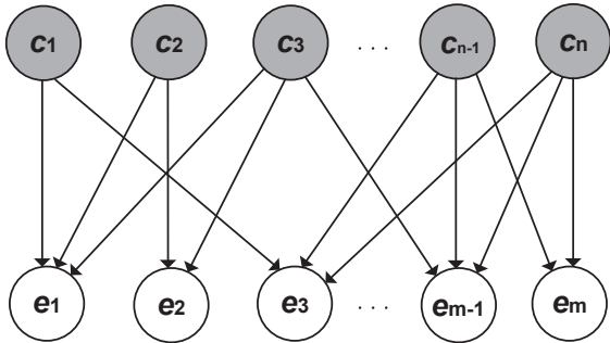
Figure 3: A concept-entity bipartite graph
