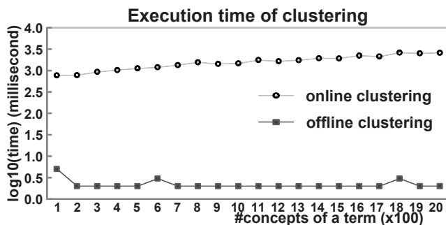
Figure 8: Execution time in online/offline clustering
