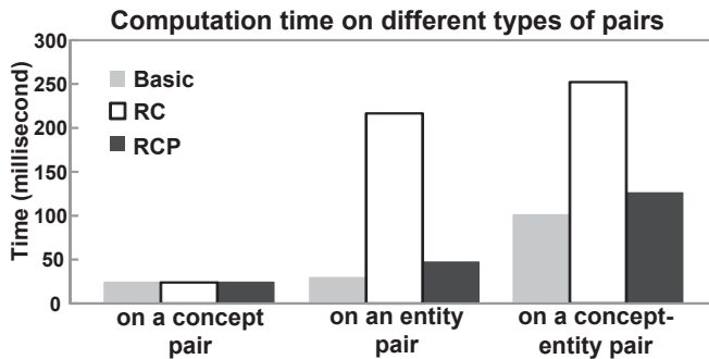
Figure 10: Computation time on different types of pairs
