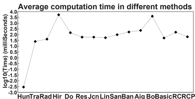
Figure 9: Computation time in different approaches
