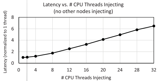
Figure 10: Latency in the pipeline increases with the number of threads due to queuing.
