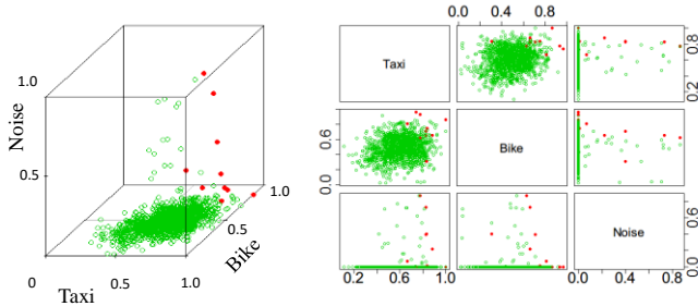
Figure 6. Aggregate multiple ods by skyline algorithms
