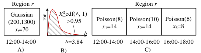
Figure 5. Illustration of applying LRT to a single dataset
