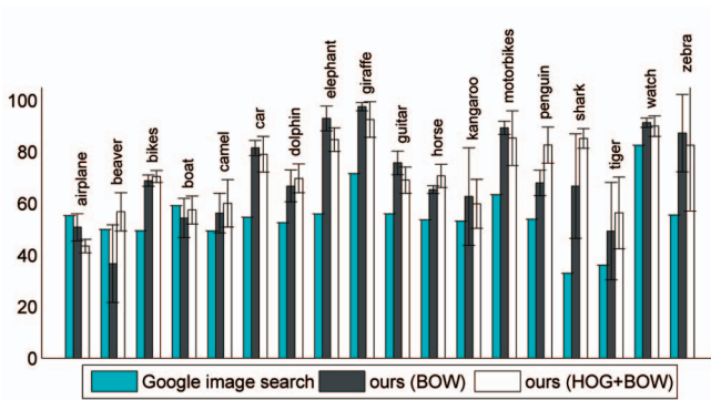
Fig. 10. Comparison with Google image search: Precision at 100 image recall. Compare to highlighted versions in first column of Table 4 for our algorithm.
