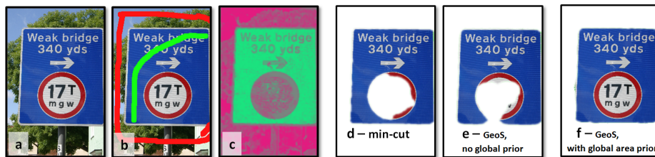
Fig. 9. Exploiting global constraints. (a) Original test image; (b) user provided F_g and B_g strokes; (c) corresponding unaries; (d) min-cut segmentation with \kappa = 0 ; The circular traffic sign is missed out. (e) GeoS segmentation on same energy as in (d); (f) GeoS segmentation on energy with global constraint G = |Area_{F_g}/Area - 0.7| .
