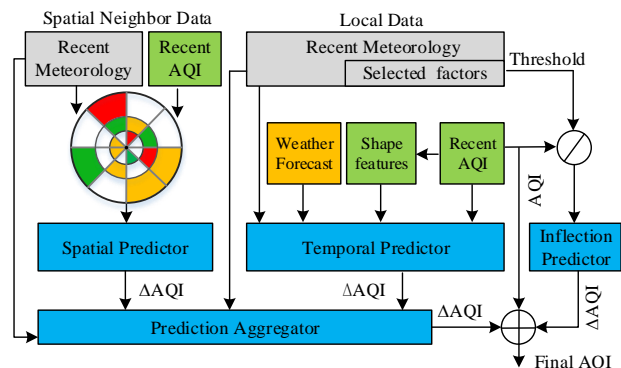
Figure 6. Framework of the predictive model
