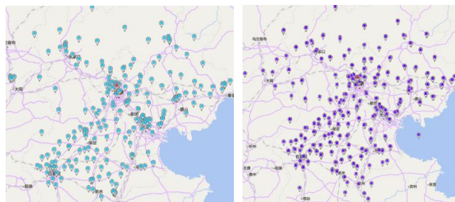
A) Nearby AQI stations for Beijing B) Meteorological sources for Beijing
