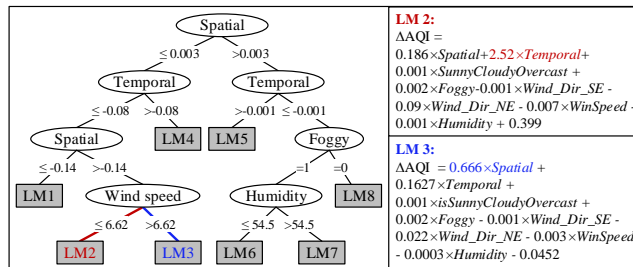
Figure 10. An example of Regression Tree
