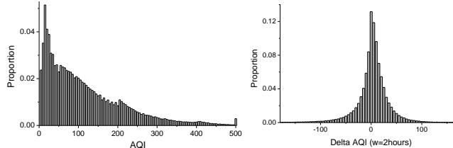
Figure 9. Distributions of AQI and in Beijing
