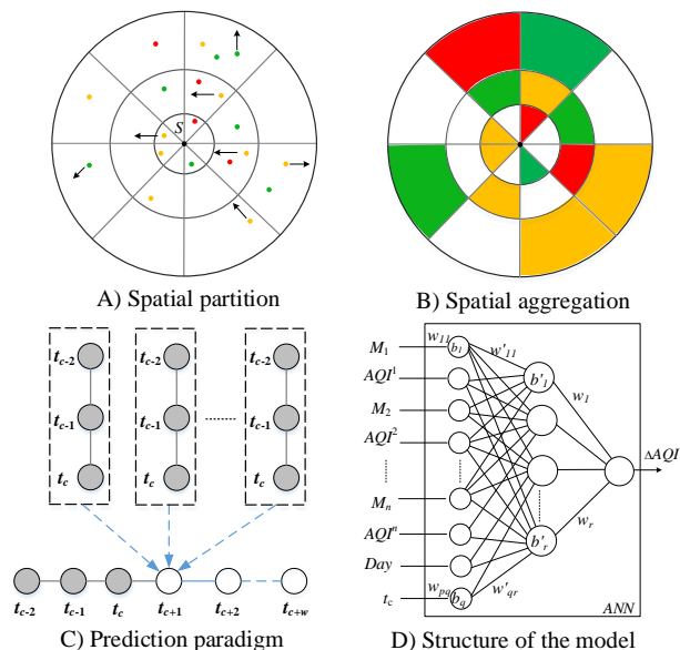
Figure 8. Illustration of the spatial predictor
