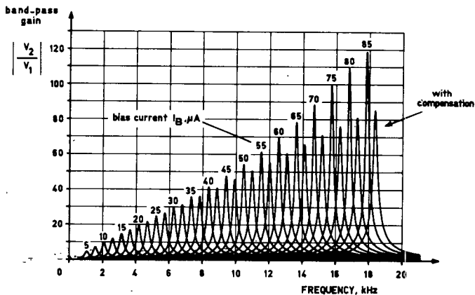
Fig. 7. Variation of the resonance frequency with constant bandwidth, in the filter of Fig. 6. The compensation capacitor eliminates the Q -enhancement effect (see text).
