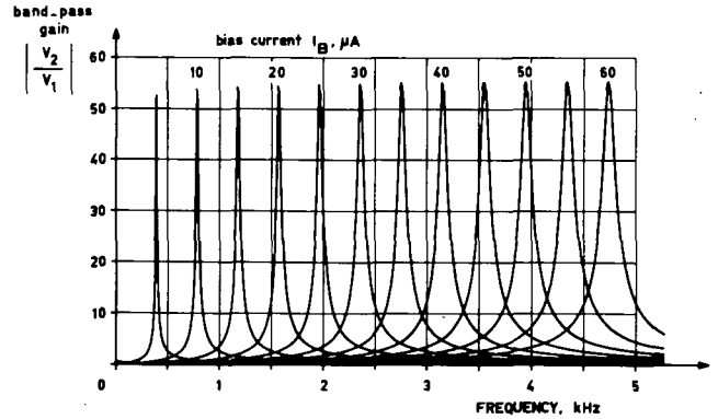
Fig. 5. Variation of the resonance frequency with I_{BQ} fixed at 2.0 \mu A for the filter of Fig. 4.
