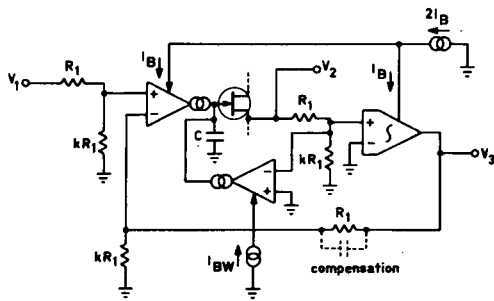
Fig. 6. This structure, similar to the filter of Fig. 4, allows the current control of the absolute bandwidth.
