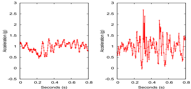
Figure 6: a_z when traversing a bump at low speed Figure 7: a_z when traversing a bump at high speed
