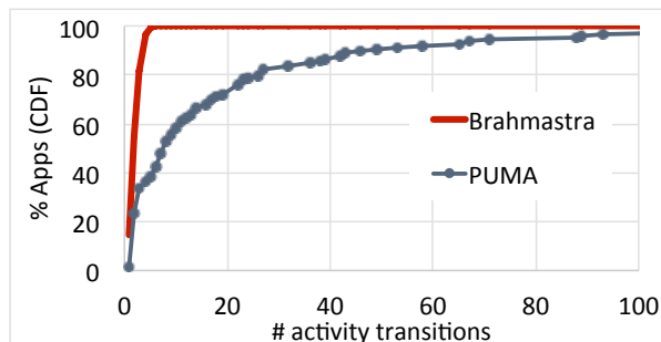
Figure 9: Test speed comparison of Brahmastra and PUMA
