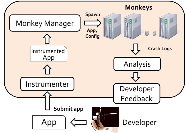
Figure 8: VanarSena Architecture.
