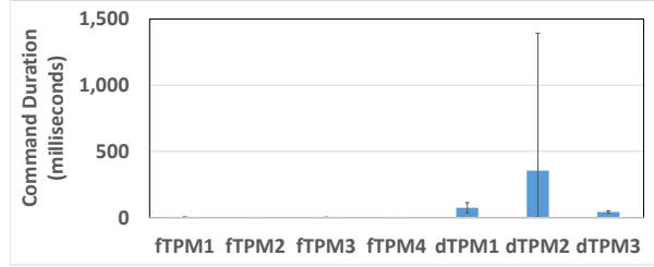
Figure 11. Performance of TPM unseal command.
