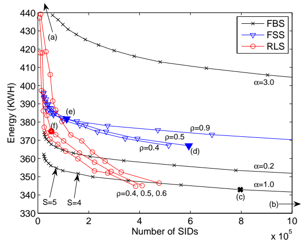
Figure 10: Energy-SID tradeoff of different algorithms with key arameters varied. The particular scenarios (c),(d),(e),(f) listed in Table 2 are labeled with bold symbols. The scenarios (a) and (b) are out of scope of this figure, but their relative locations are pointed by arrows.
