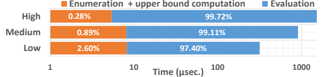
Figure 5: Average running time of “query enumeration + upper bound computation” v.s. “query evaluation” per PJ query
