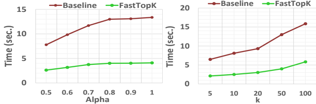
(a) Varying score weight \alpha
